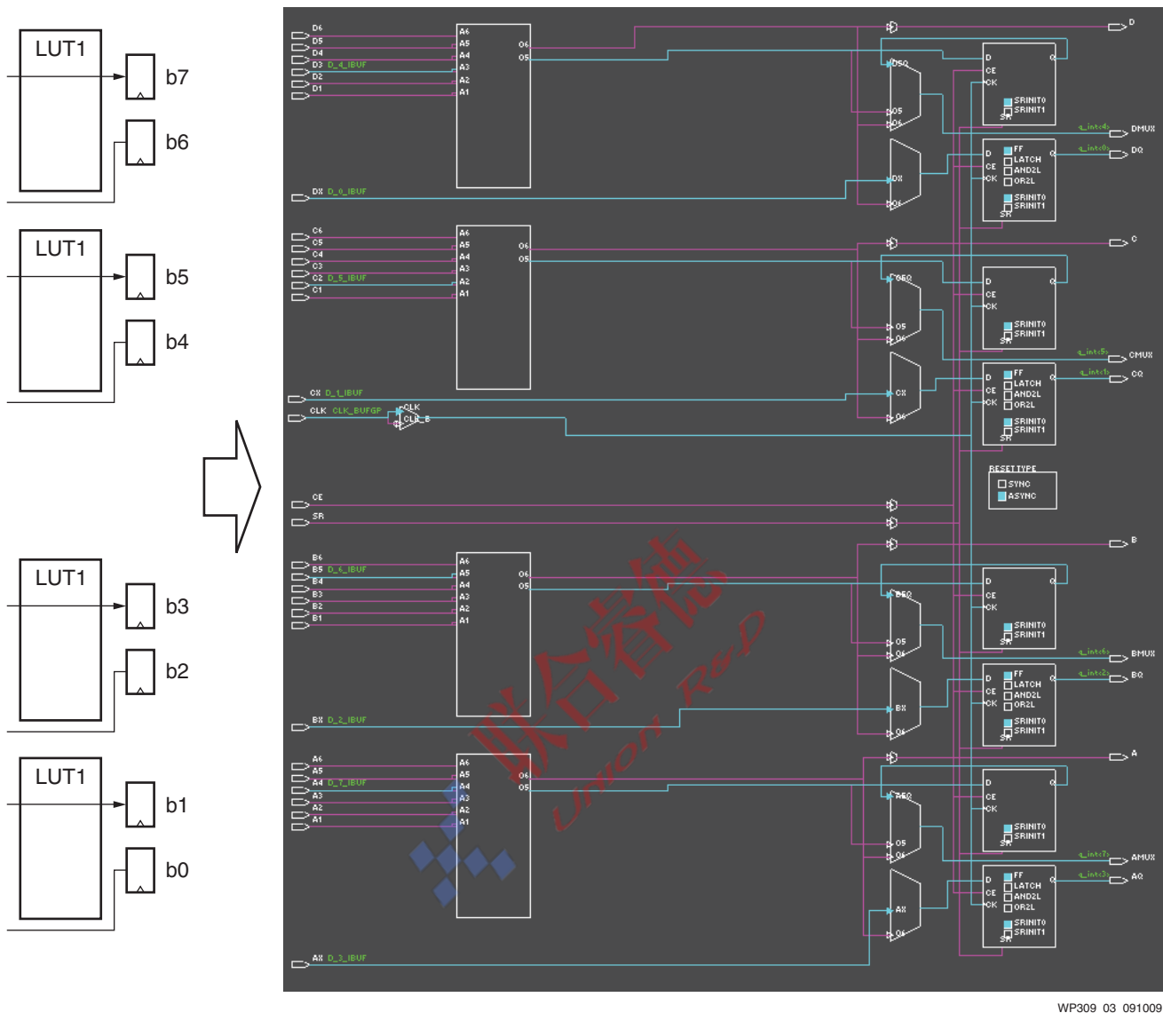
Figure 3: FPGA Editor Representation of a Route-Thru
